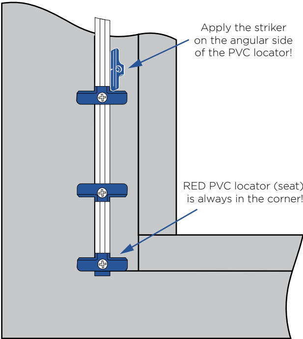
CAM scheme
