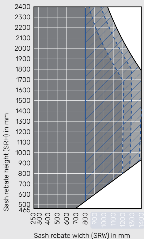
APPLICATION DIAGRAM
